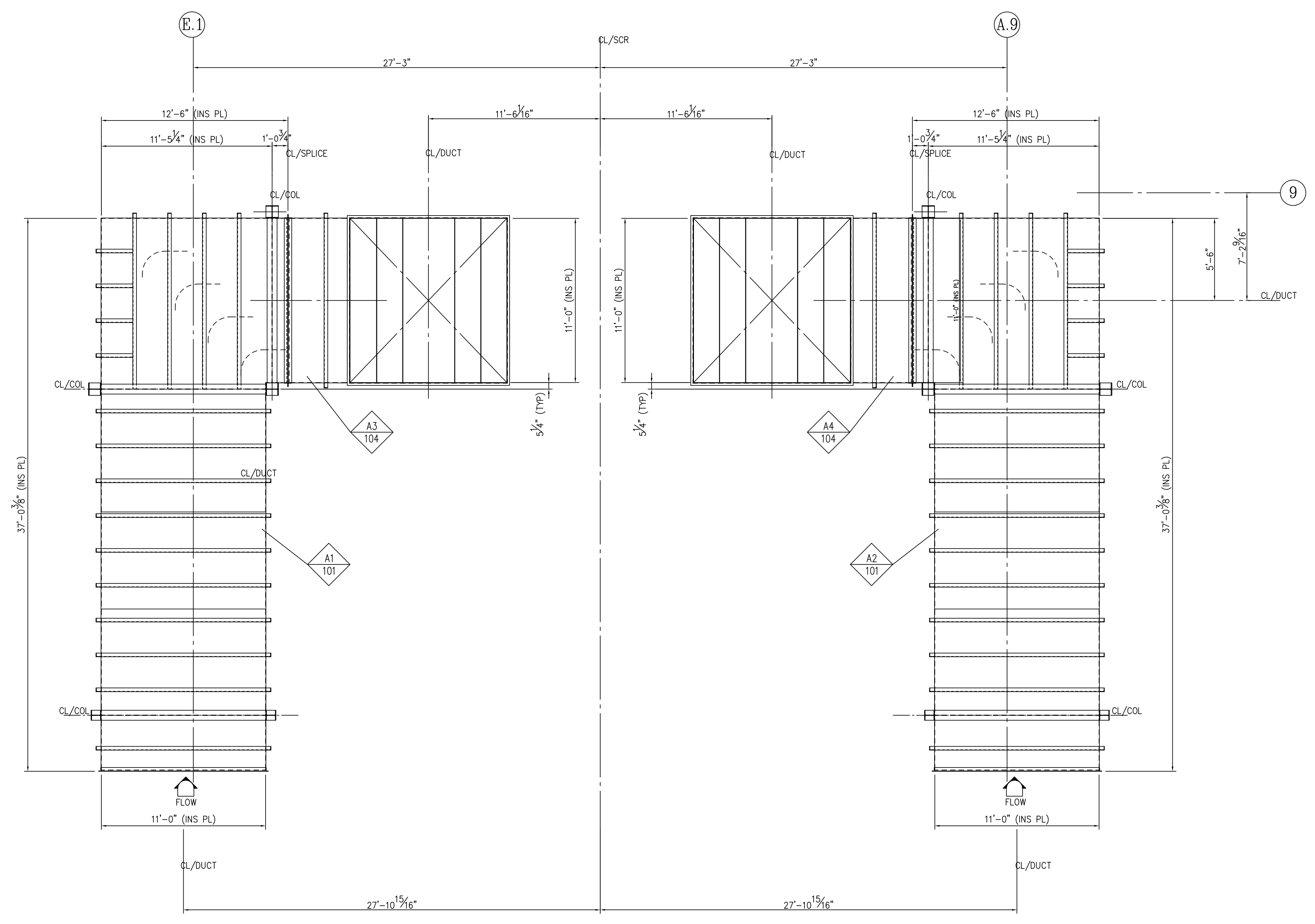
DUCT "B" TOP PLAN VIEW
