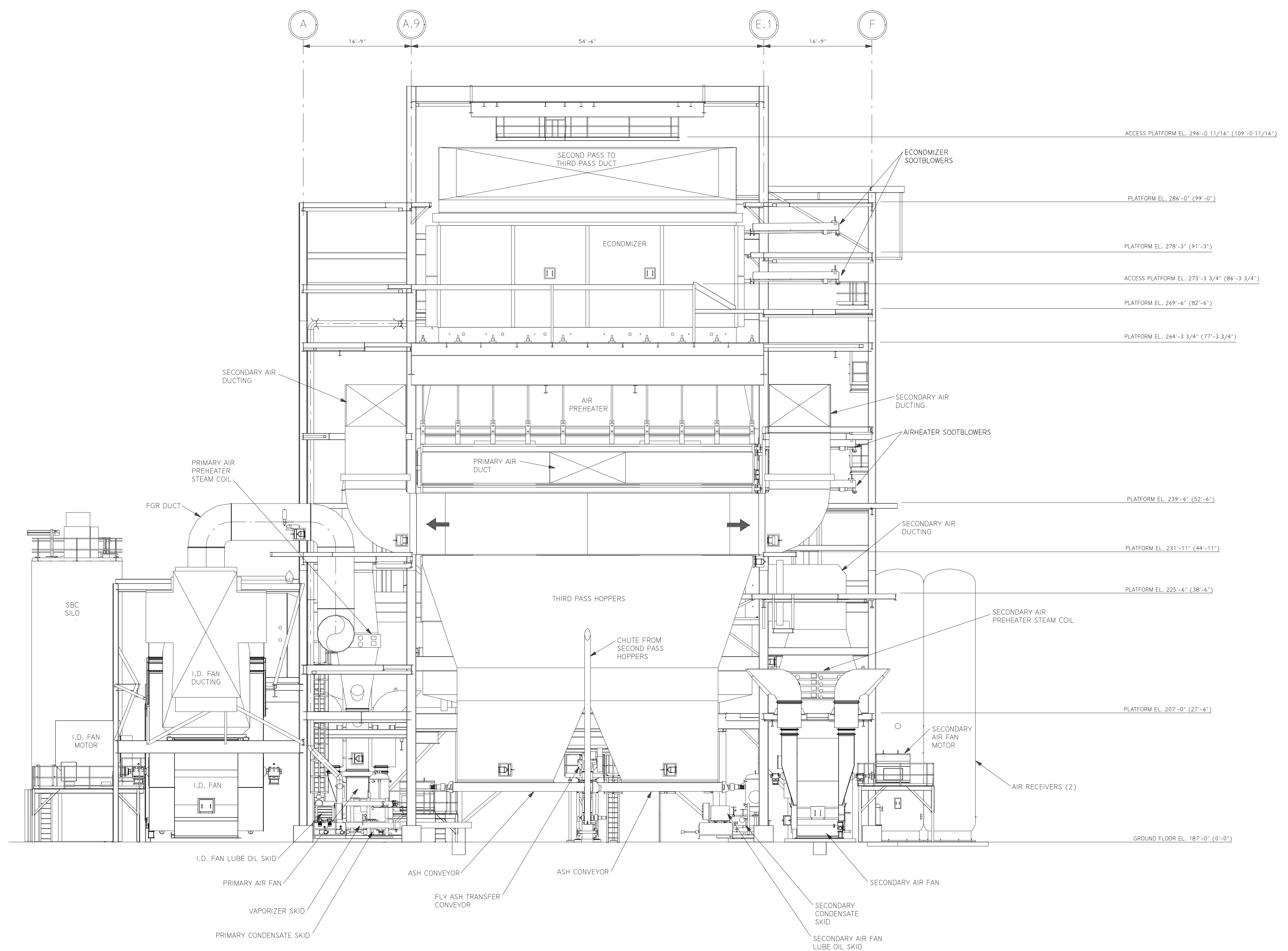
SECTION B-29534 LOOKING SOUTH 29547
