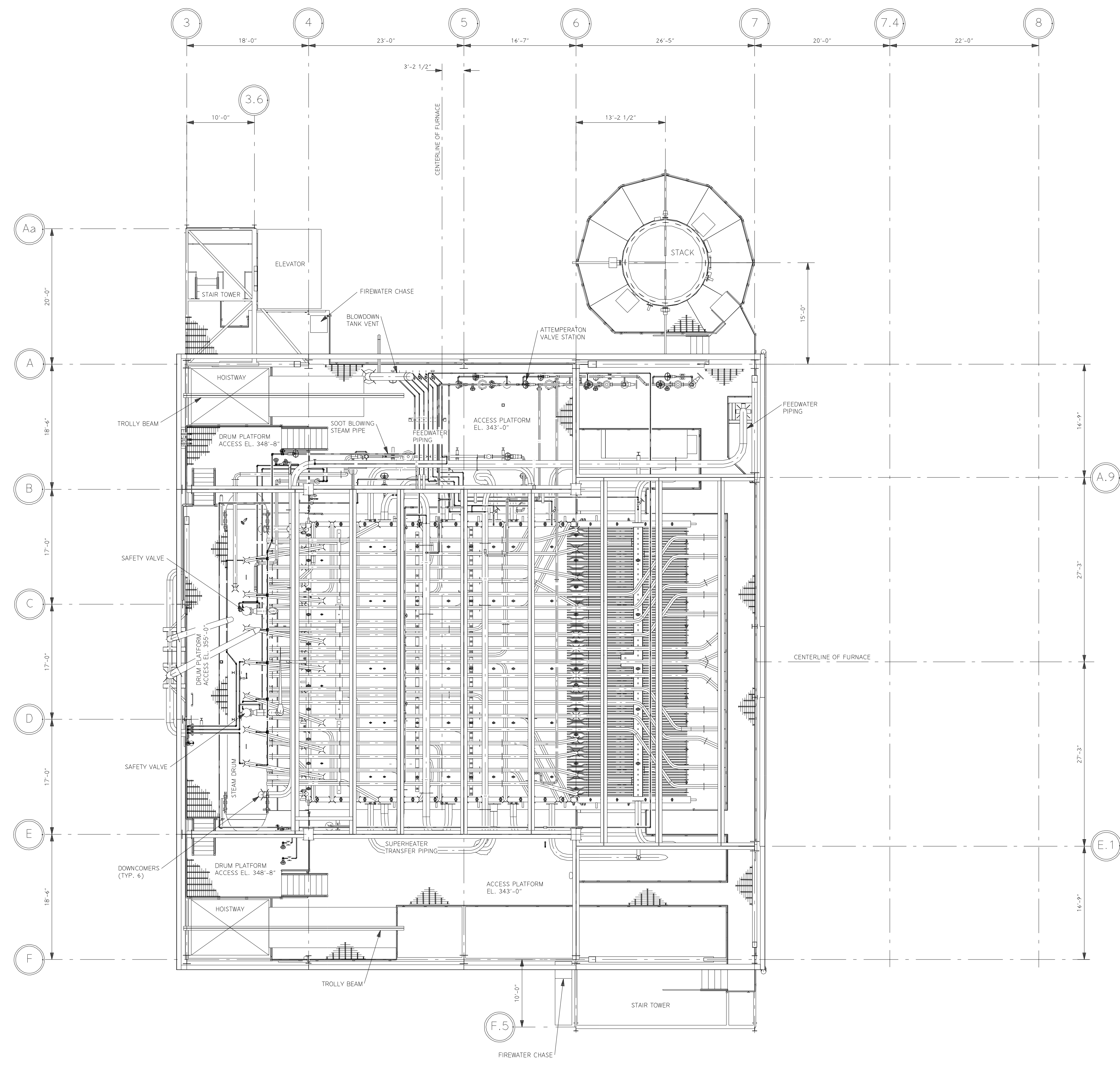
PLAN VIEW ELEVATION 343'-0", 348'-8" & 355'-0"
